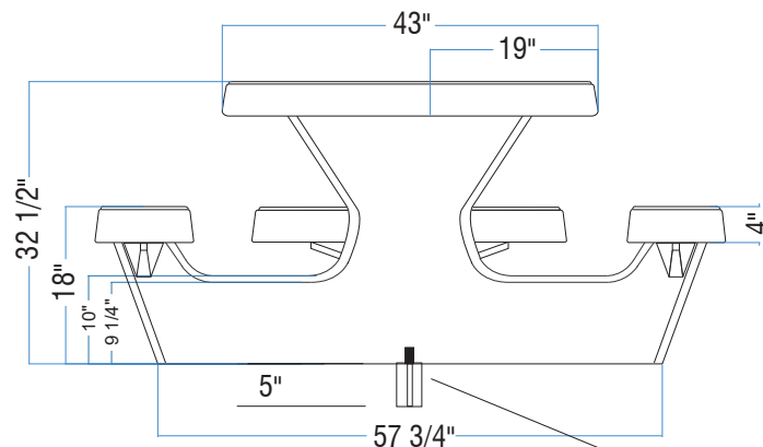
SECOND SIDE ELEVATION
