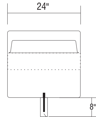
SECTION
