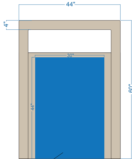
ELEVATION (Door Open)
