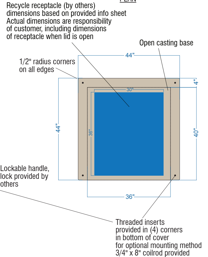
PLAN
