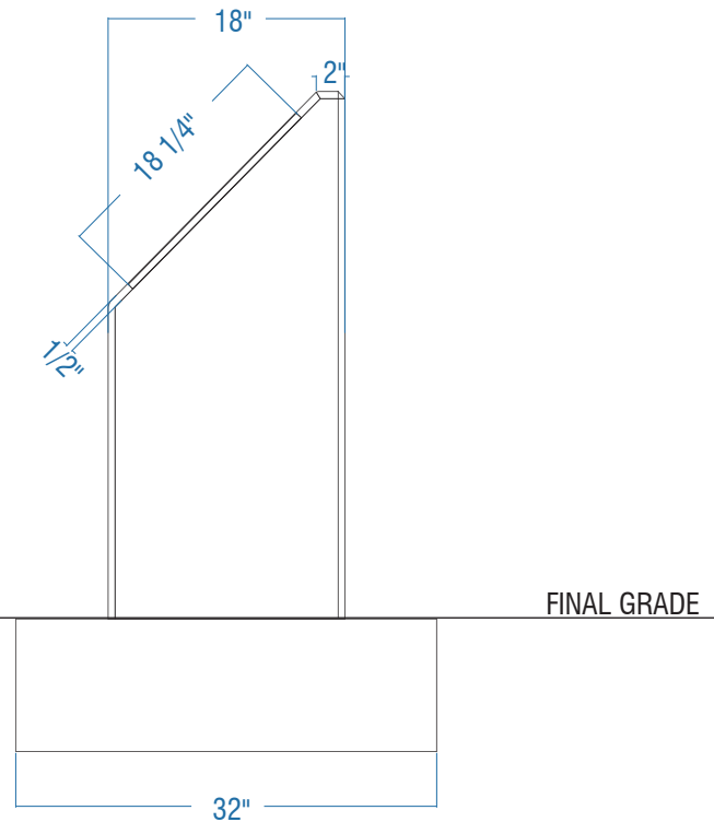
SIDE ELEVATION
